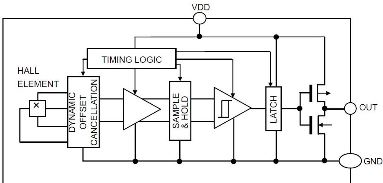
Figure 3, Block Diagram of AS1812
