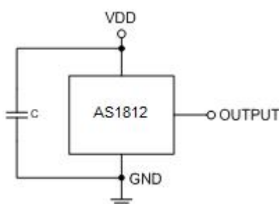
Figure 1, Typical Application Circuit of AS1812
