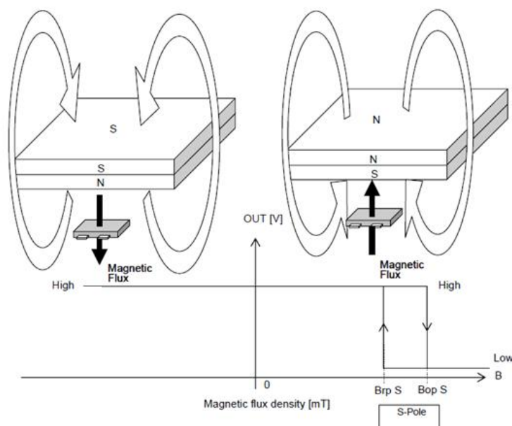
Fig 4, Magnetic Operation Characteristic of AS1812
